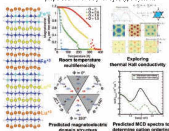
A non-polar lattice distortion driven various properties in \text{LuFeO}_3/\text{LuFe}_2\text{O}_4 type systems
