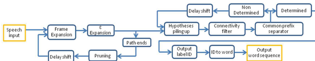
図 2 Pipeline based design of a speech decoder.
