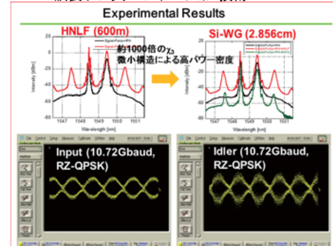
図6 FWM波長変換特性(HNLF・Si細線導波路)
