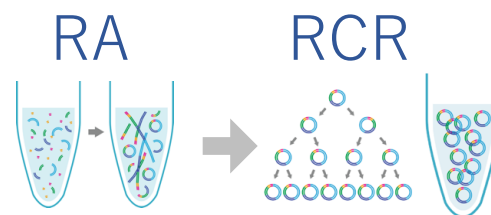
Fig.2 Two step cell-free cloning using RA-RCR
